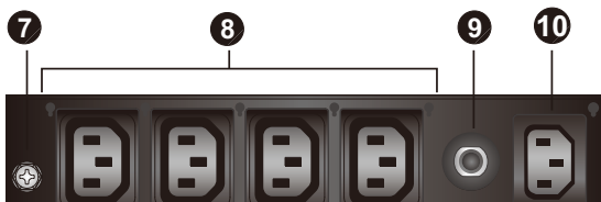
PE4104G (Rear View)
