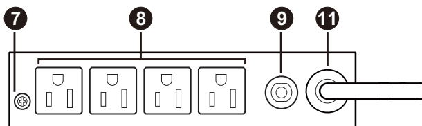
PE4104A / PE4104AJ (Rear View)
